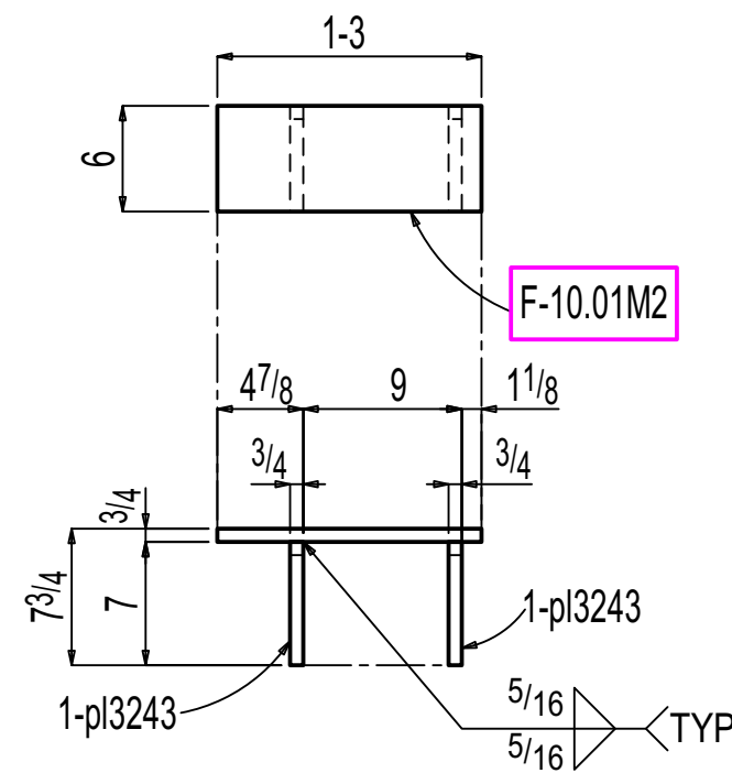
ONE PLATE F-10.01M2
