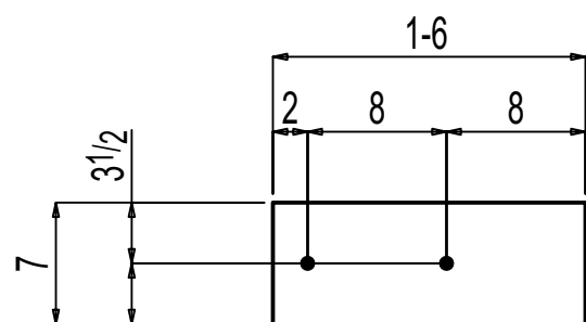
ONE LEVELING PLATE F-10.01LP1
