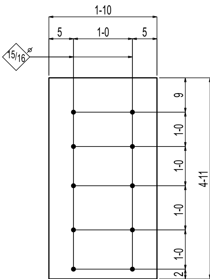
ONE EMBED PLATE F-10.01EP1
