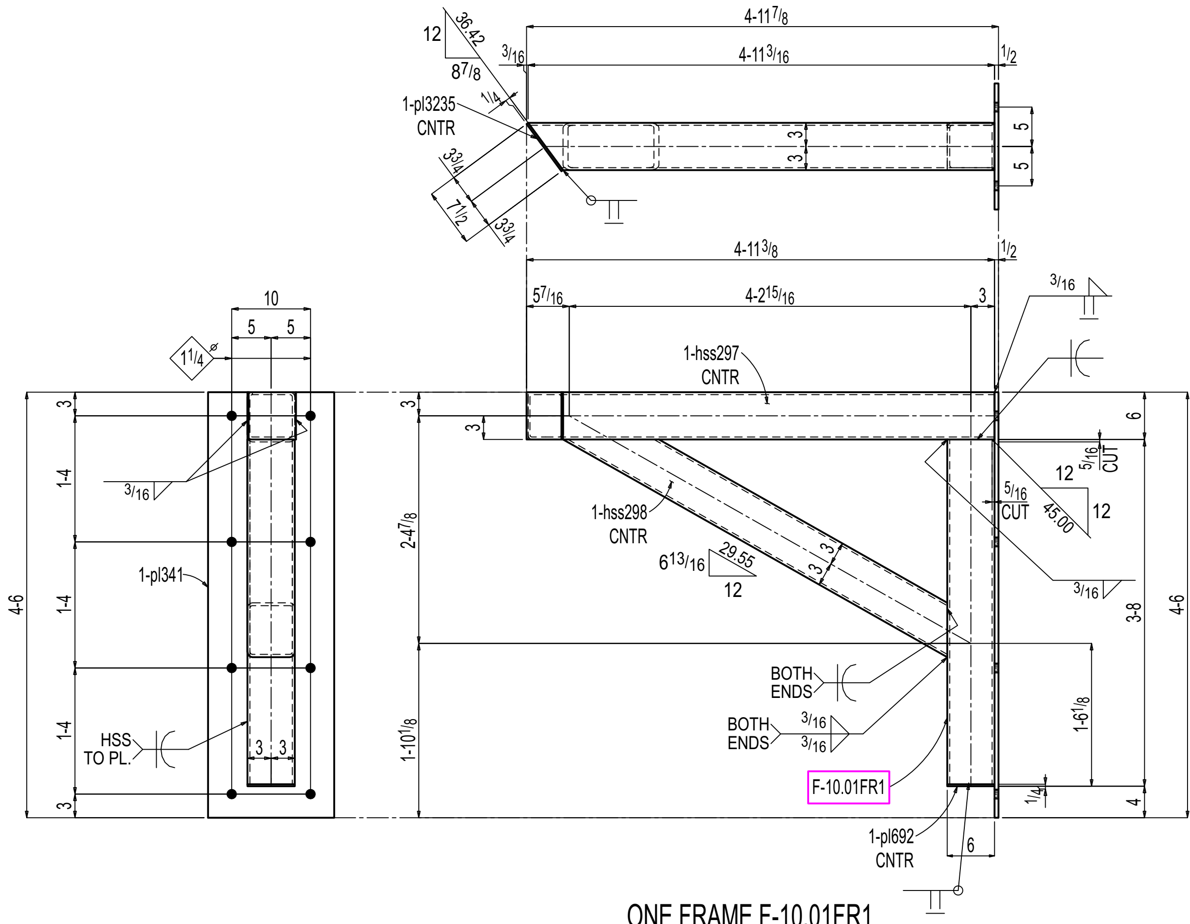
ONE FRAME F-10.01FR1
