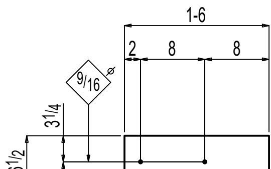
ONE LEVELING PLATE F-10.01LP2
